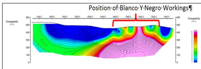
Figure 2: Pole-Dipole IP Chargeability over Blanco Y Negro Workings
