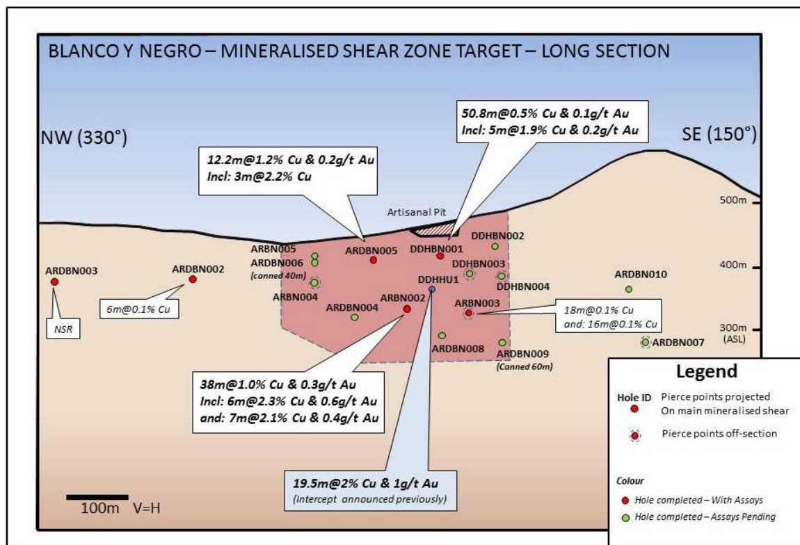
Figure 1: Longsection of the Blanco Y Negro Prospect
